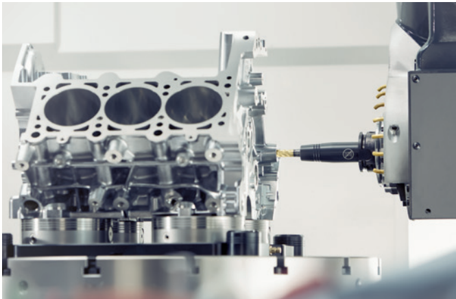
Cylinder head machining with the TENDO Slim 4ax
